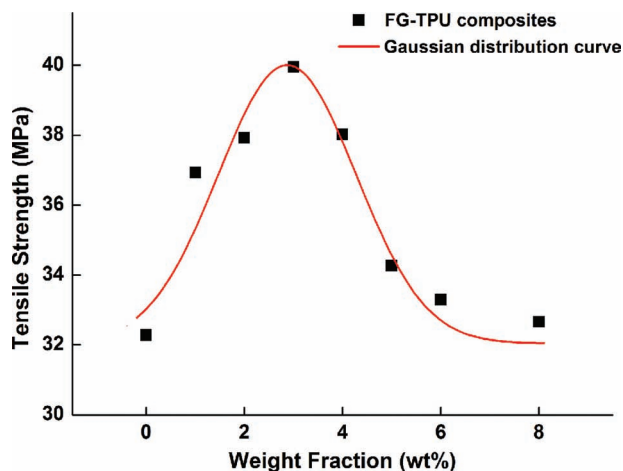
Figure 1. Tensile strengths of the FG-TPU composites with different FG loadings.
