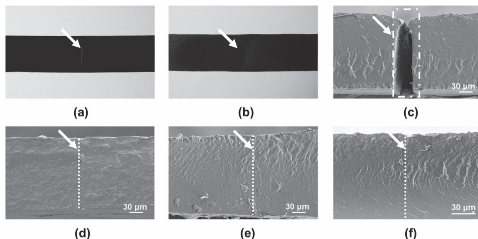
Figure 3. Optical and SEM images of the fractured sample with 6 wt% FG loading before and after healing. a,b) The optical images of the fractured sample before a) and after b) IR light healing. c-f) The cross-sectional SEM images of the fractured samples before c) and after IR light d), electricity e), electromagnetic wave f) healing, respectively.
