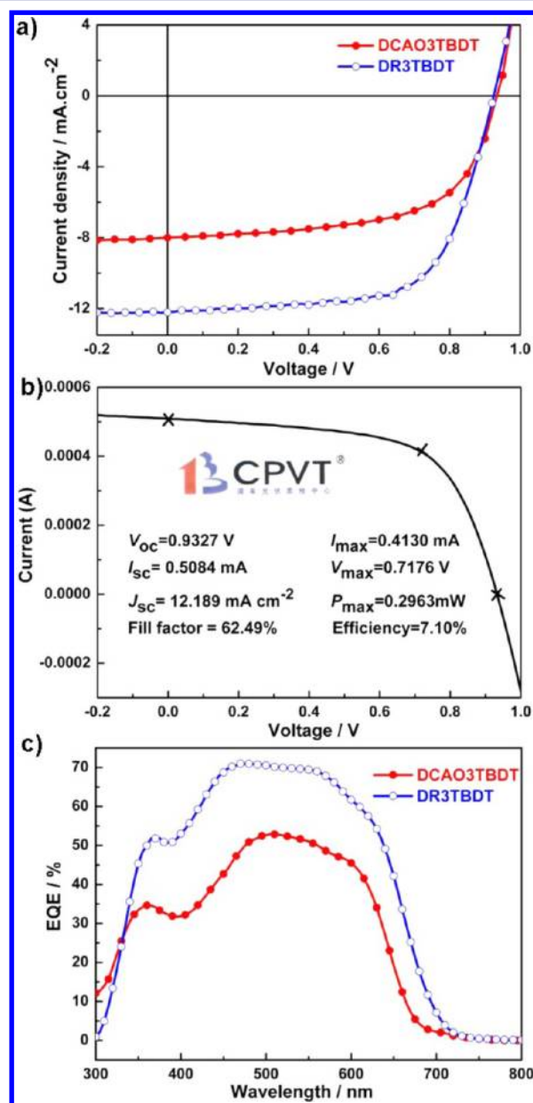
Figure 3. (a) J - V curves of solar cells with an active layer composed of DCAO 3 TBDT/PC 61 BM (1:0.5, w/w) and DR 3 TBDT/PC 71 BM (1:0.8, w/w) with 0.2 mg mL -1 PDMS; (b) the certified performance of a device based on DR 3 TBDT/PC 71 BM with 0.2 mg mL -1 PDMS; (c) EQE plots of solar cells with an active layer composed of DCAO 3 TBDT/PC 61 BM (1:0.5, w/w) and DR 3 TBDT/PC 71 BM (1:0.8, w/w) with 0.2 mg mL -1 PDMS.
