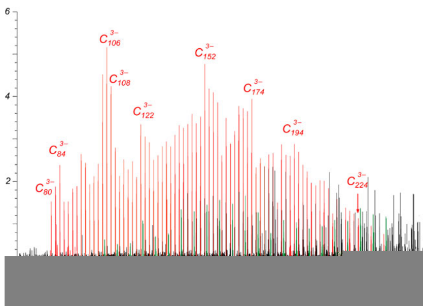
Figure 4. Mass spectra of negative carbon clusters in the low m/z region produced by laser ablation of G with a relative laser power of 28%. The strong signals of singly charged anions are removed in order to clarify the spectrum
