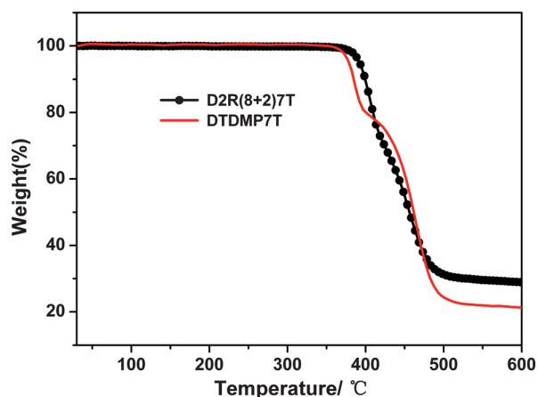
Fig. 1 TGA plot of D2R(8 + 2)7T and DTDMP7T.
