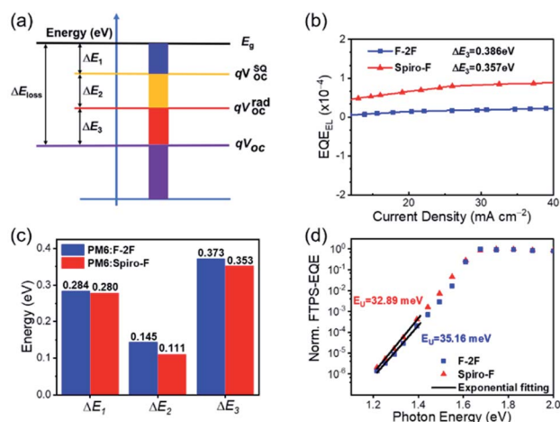
Fig. 5 (a) The total energy losses analysis in OSCs. (b) \text{EQE}_{\text{EL}} of the devices based on the as-cast PM6:F-2F and PM6:Spiro-F blended films. (c) Radiative and non-radiative energy losses in the OSCs studied here. (d) FTSP-EQE of the PM6:F-2F and PM6:Spiro-F based devices at the absorption onset.
